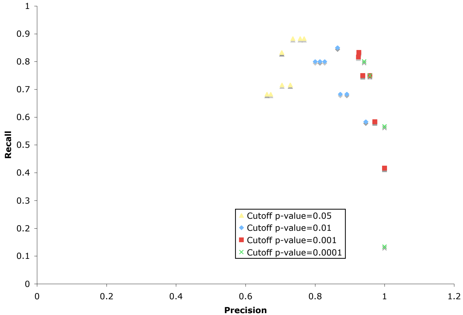
Precision-recall plot at different significance cutoffs (based on FP/FN rate of 5%)
