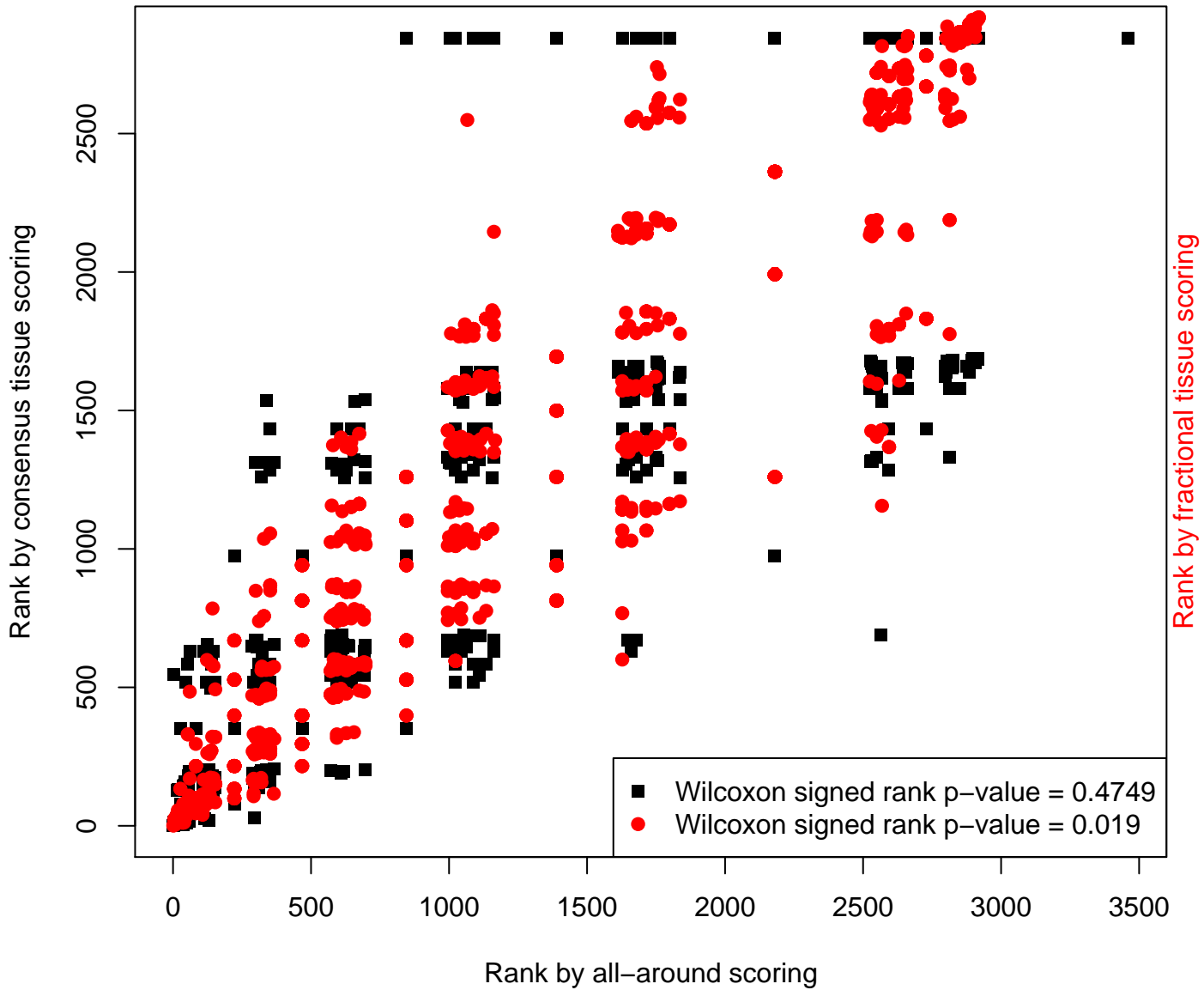
Comparison of the ranks of groups in all three scoring schemes
