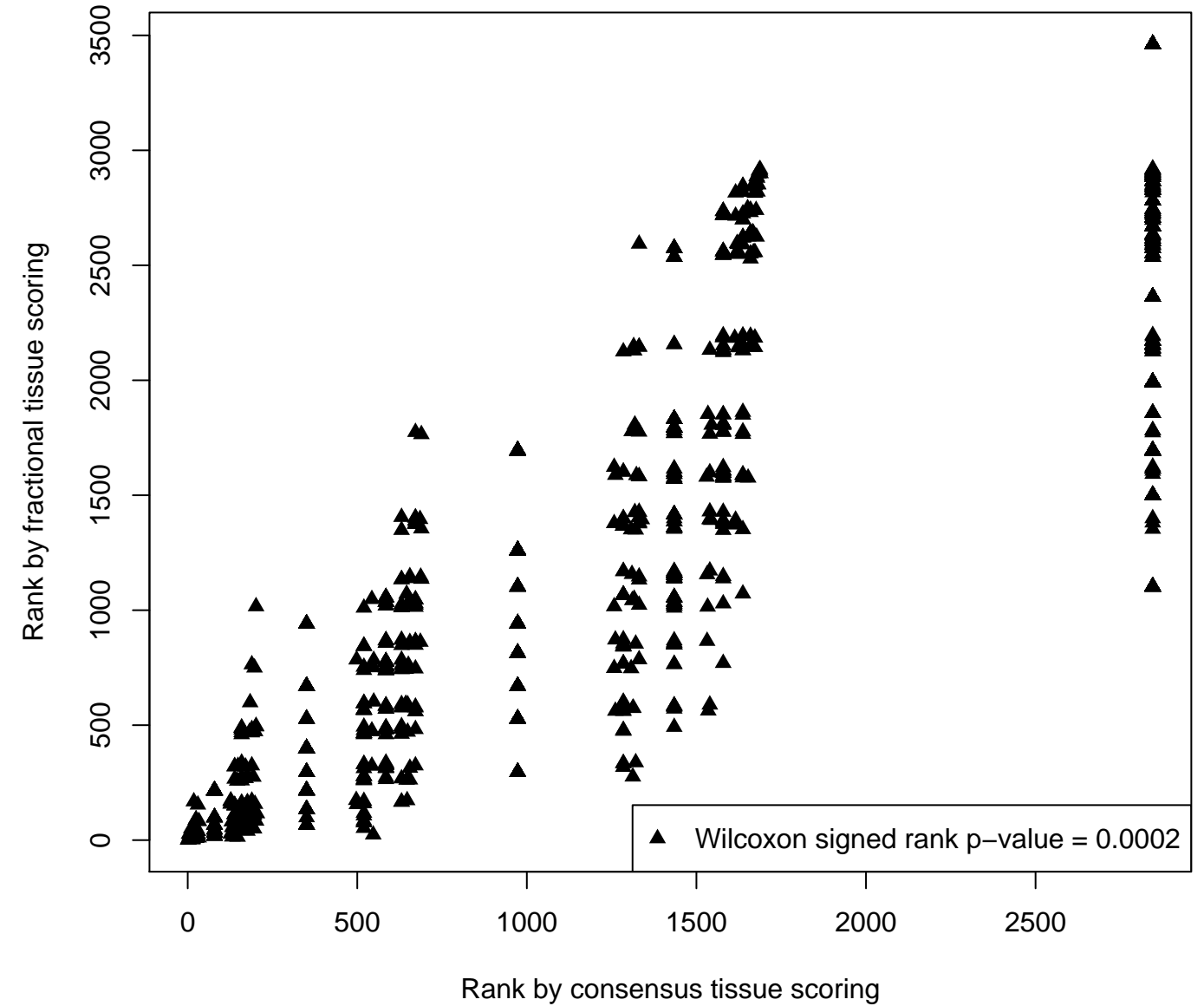
Comparison of the ranks of groups in tissue scoring schemes
