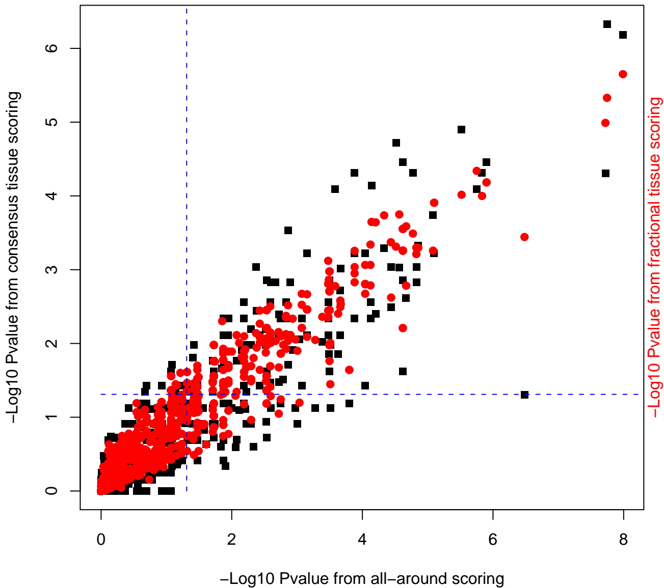
Log-log plot of the p-values for the three different scoring schemes
