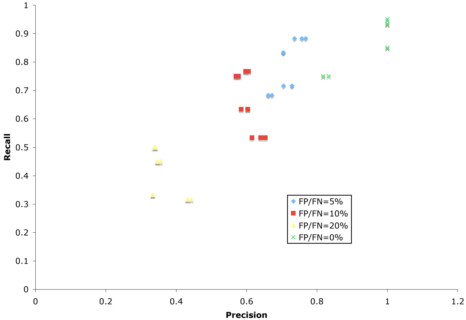
Precision-recall plots for different FP/FN rates of simulation data
